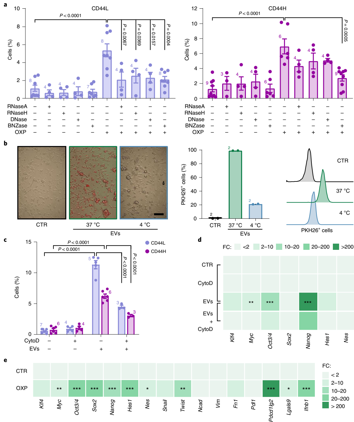
Fig. 3 | Cell-to-cell horizontal transfer of nucleic acids and dedifferentiating factors during immunogenic chemotherapy. a , Multiparametric flow cytometry analysis of CSC surface markers in receiving viable MCA205 cells upon coculturing with donor MCA205 cells left untreated or previously treated with OXP (300 \mu M, 24 h) alone or in combination with the indicated nucleases. Columns represent the percentage of CD44H and CD44L cells, expressed as mean \pm s.e.m. and individual data points. Number of biologically independent experiments are reported. b , Fluorescence microscopy (left) or flow cytometry (right) analysis of the internalization (at 37 °C and 4 °C) of donor cell-derived, PKH26-stained EVs by receiving MCA205 cells. Scale bar, 100 \mu m. One representative experiment out of two is shown. c , Multiparametric flow cytometry analysis of CSC surface markers in receiving MCA205 cells cocultured with donor MCA205 cell-derived EVs in the presence of cyto D (0.5 \mu M). Data are expressed as mean \pm s.e.m. and individual data points; number of biologically independent experiments is reported. d,e , Assessment of the expression levels of the indicated reprogramming factors by qRT-PCR in receiving MCA205 cells stimulated with donor MCA205 cell-derived EVs alone or in the presence of cyto D, as before ( d ) and inside EVs ( e ). Data are reported as mean FC \pm s.e.m. over control conditions, n=2 and n=3 , for d , n=2 , n=3 , n=4 , n=6 , n=7 , n=9 and n=10 for e , independent experiments, after intrasample normalization to Ppia expression levels. * P < 0.05 , ** P < 0.01 , *** P < 0.001 , see Supplementary Table 1 for exact P values. See also Extended Data Fig. 3. a,c,d , Ordinary one-way ANOVA test followed by Bonferroni's correction. e , Unpaired two-sided Student's t -test.
